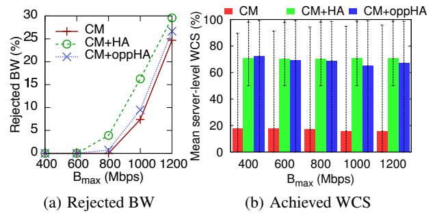
Figure 12: Comparison of different HA mechanisms. CM: default approach w/o any HA. CM+HA: guarantee 50% WCS. CM+oppHA: opportunistic HA.
