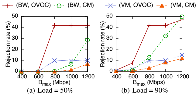
Figure 7: Rejection rates with various bandwidth scaling. Legend format: (metric, algorithm).
